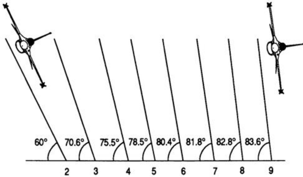
Required G Forces to Maintain Bank
