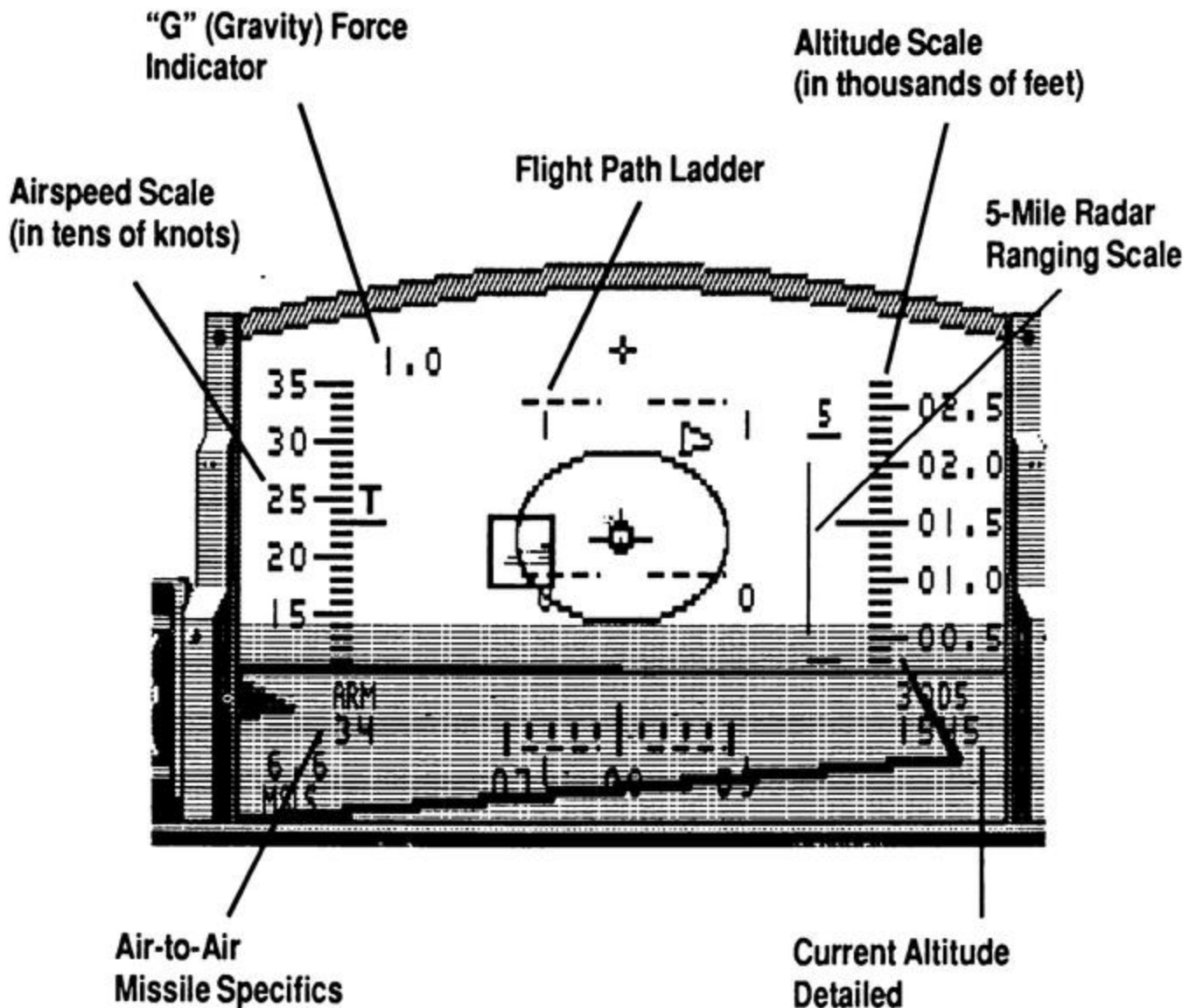
HEAD-UP DISPLAY (HUD) IN "AIR-TO-AIR" MODE
