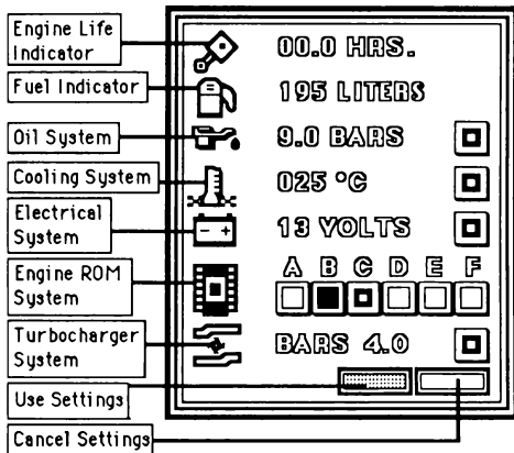
Figure 11: Engine Control
