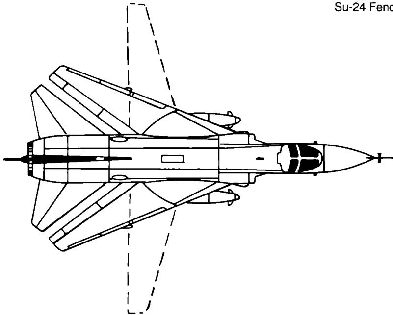
Su-24 Fencer
