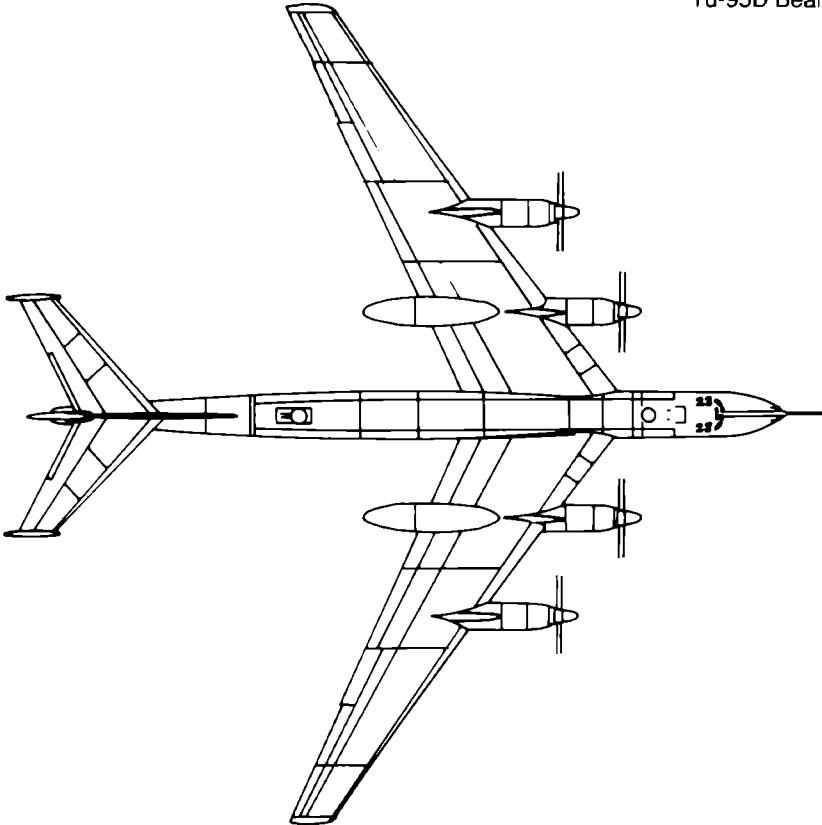
Tu-95D Bear
